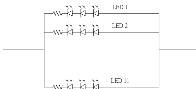
LED Light Bar Circuit
