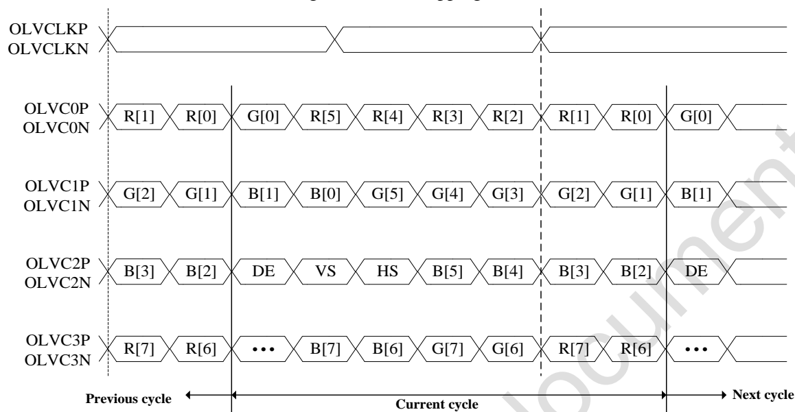
Figure 11 Date Mapping(8 Bit)
