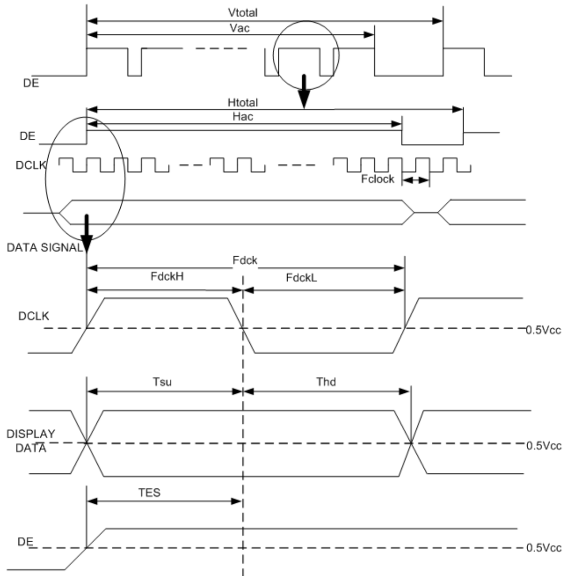
Figure 14 Timing Characteristics
