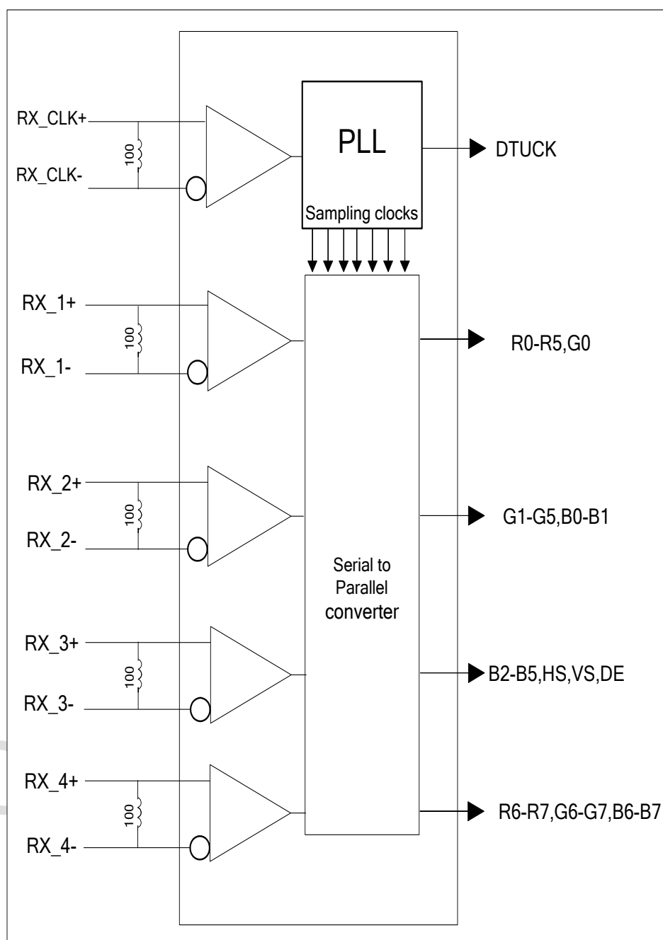
Figure 13 LVDS Receiver Internal Circuit
