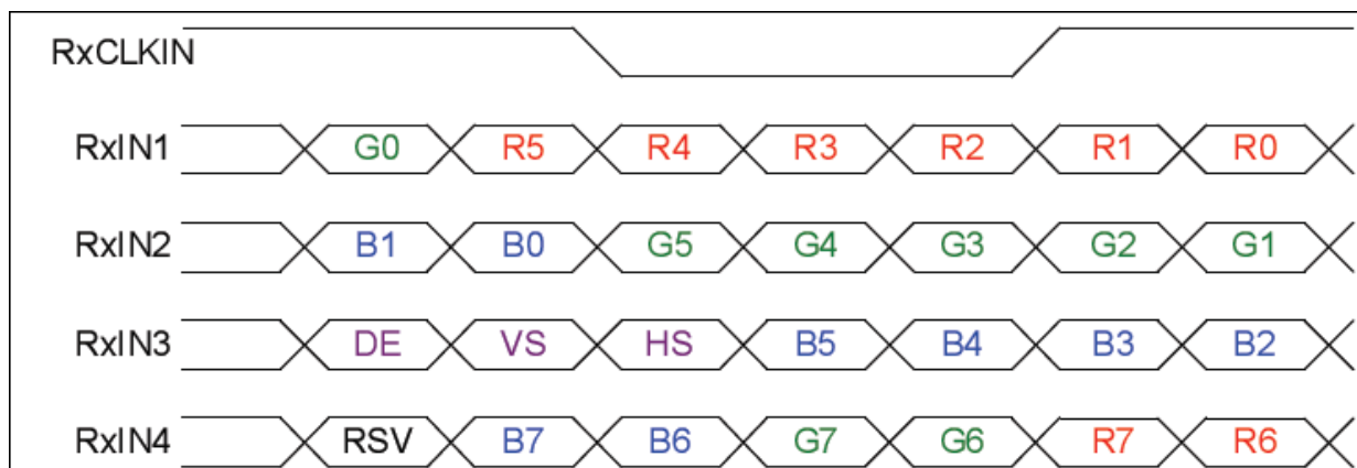
Figure 6 Timing Characteristics
