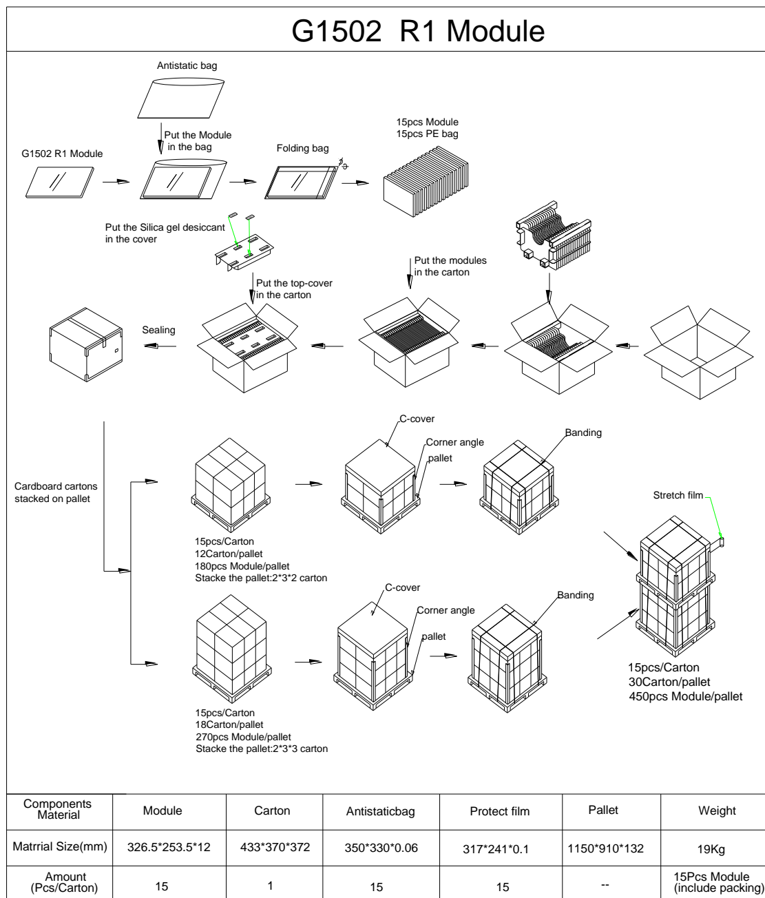
Figure 20 Packing Method
