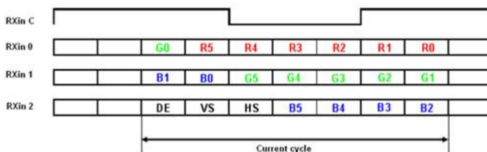
Figure 8 Timing Characteristics
