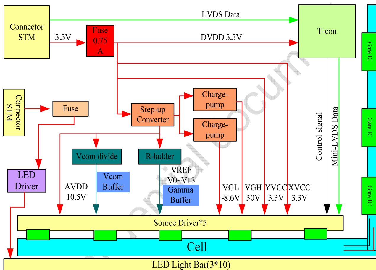
Figure 1 Block Diagram
