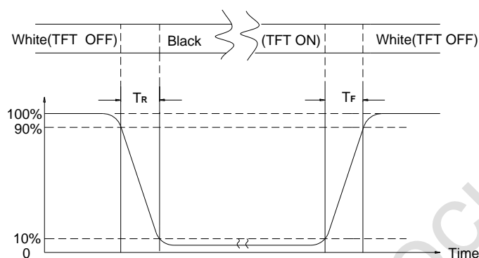
Figure 5 Definition of Response Time
