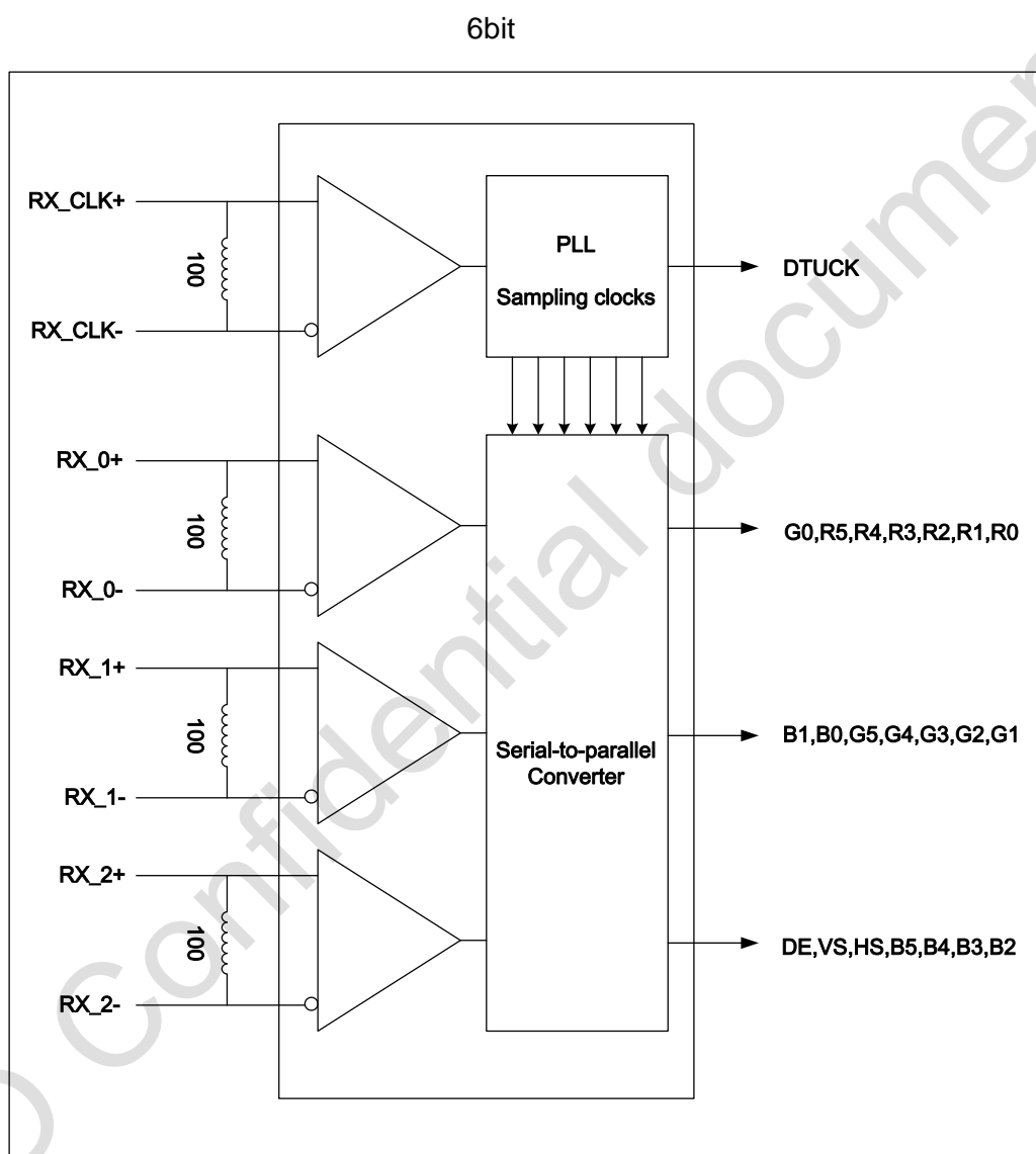
Figure 10 LVDS Receiver Internal Circuit
