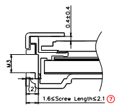
SECTION A-A SCALE 5/1
