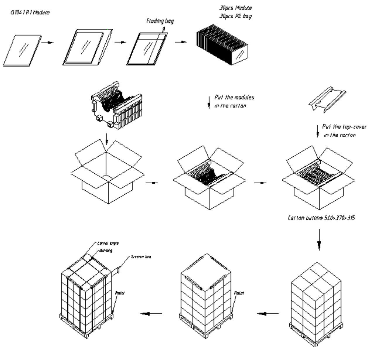
Figure 19 Packing Method
